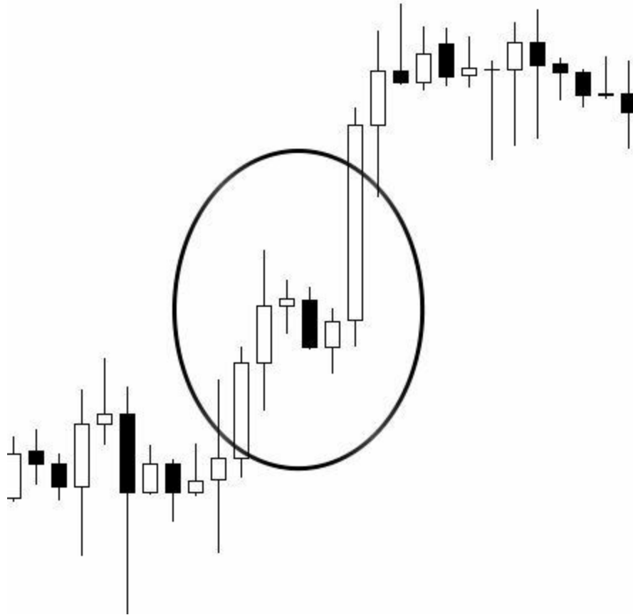
Diagram 5-5: Shallow Pullback
