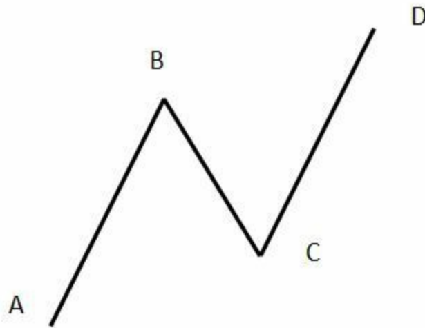
Diagram 6-1: Simple Pullback
