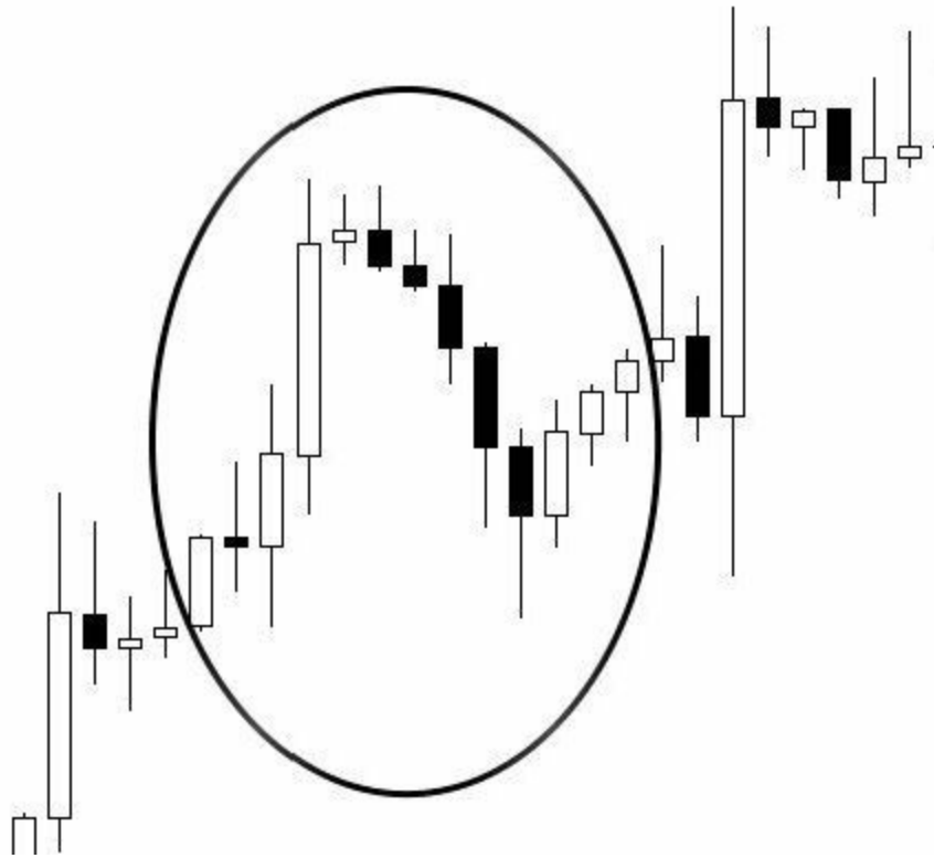
Diagram 5-4: Deep Pullback
