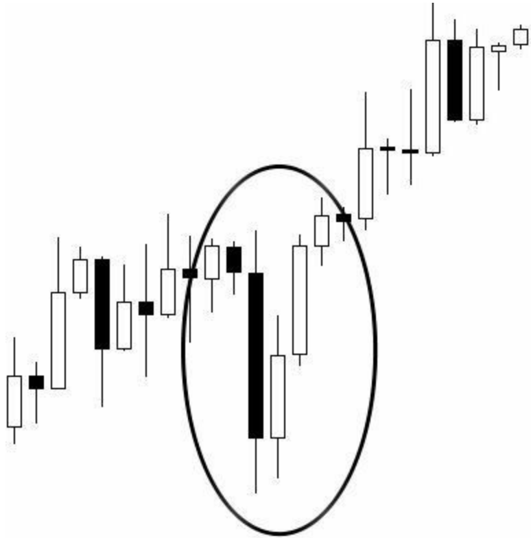
Diagram 5-6: Sharp Pullback
